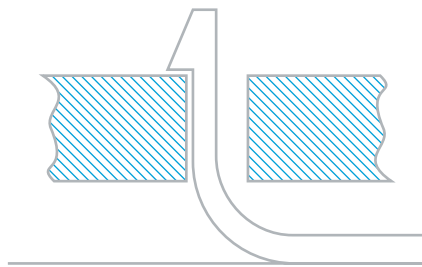
Figure 4. L-shaped snap-fit assembly operation
