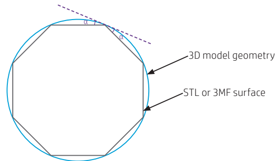
Figure 4. Angle tolerance
