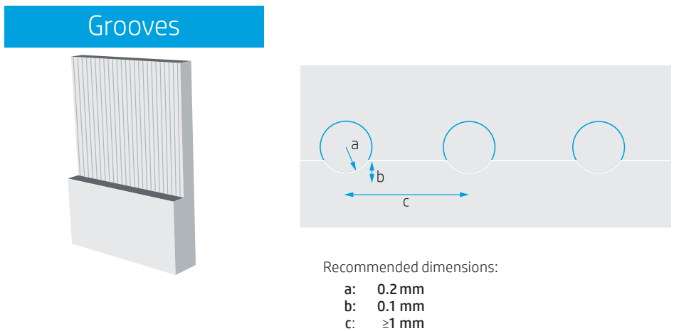
Figure 13: Grooves to increase bonding area: Design recommendations
